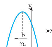
f(x) = ax^2 + bx + c, a < 0
